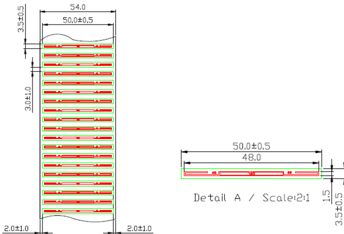
Wet Inlay Roll Dimensions
