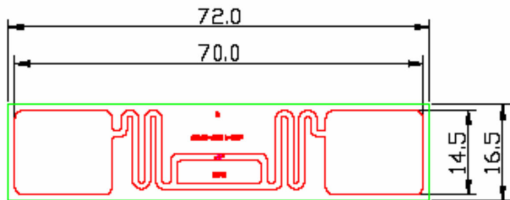
Wet Inlay General Dimensions
